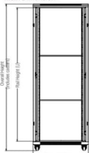
Front View Without front door
